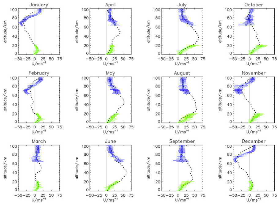
Fig. 4. As Fig. 3 but for Rothera zonal winds.
