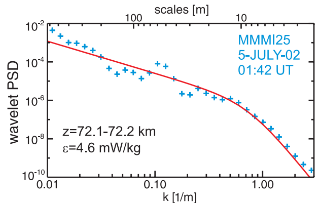
Figure 2. Power spectrum as a function of wavenumber (lower abscissa) observed at \sim 72 km altitude during the flight MMMI25 (blue symbols). The red solid line shows the corresponding best fit by a Heisenberg-spectrum, yielding an \epsilon -value of 4.6 mW/kg. The upper abscissa converts wavenumbers to spatial scales.
