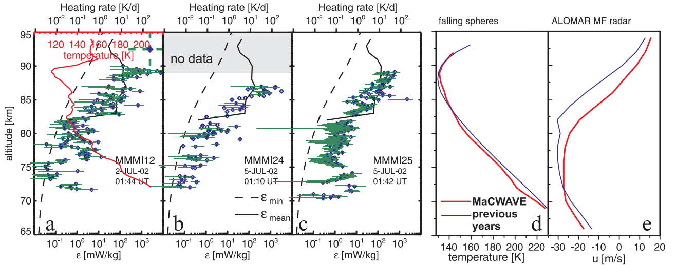
Figure 1. Panels a-c: Turbulent energy dissipation rates \epsilon (blue symbols, lower abscissa) and errors (green horizontal bars) as a function of altitude for the sounding rocket flights MMMI12, MMMI24, and MMMI25. The uppermost abscissa converts \epsilon to heating rates. The dashed line indicates a gross-estimate of the ‘minimum’ turbulent energy dissipation rate \epsilon_{min} (see text). The solid black line indicates the mean \epsilon -profile ( \epsilon_{mean} ) derived from ten former sounding rocket flights in summer [Lübken et al. , 2002]. The red line (panel a, red upper abscissa) shows the temperature profile measured during flight MMMI12, and the grey shaded area in the panel b indicates the low apogee of only 89.2 km during flight MMMI24 (see text). Panels d and e show mean temperatures and zonal winds from MaCWAVE/MIDAS (red) and previous years (blue), reproduced from Goldberg et al. [2004] and Singer et al. [2004].
