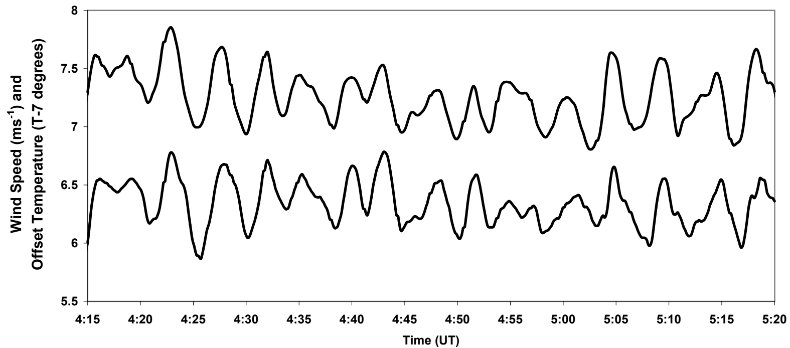
14 October 1999 (Flight #7 Package #1): 60-sec Averaged Horizontal Wind Speed and Offset Temperature (T-6degrees)
