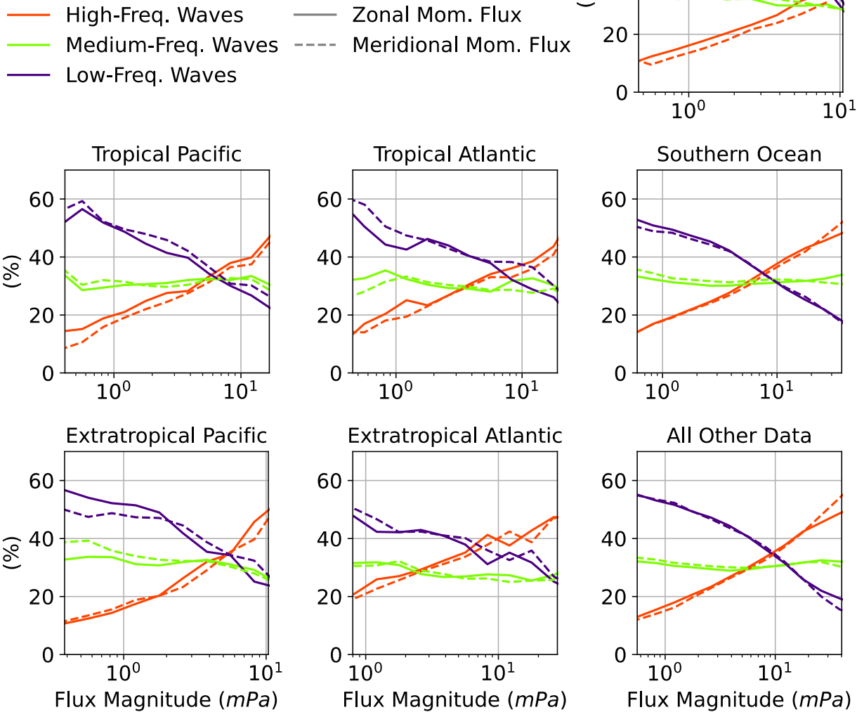
Figure 8. The fraction of the magnitude of the zonal (solid curves) and meridional (dashed curves) momentum fluxes due to high-, medium-, and low-frequency waves. The flux magnitudes are calculated by setting all component (northward, southward, eastward, and westward) flux time series to be positive and taking their sum, eastward + westward in the zonal direction, and northward + southward in the meridional direction. This is equivalent to taking the absolute value of the wavelet coefficients in Figure 1. We then bin the data by the flux magnitude for each region and calculate the average percent of that flux contributed by waves in each frequency band. The “All Other Data” region represents all the data gathered outside the colored regions in Figure 3 (1757817 data points).
