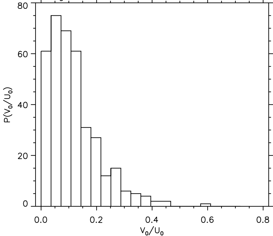
Turning-Shear Ratio PDF for < 16 km Altitude
