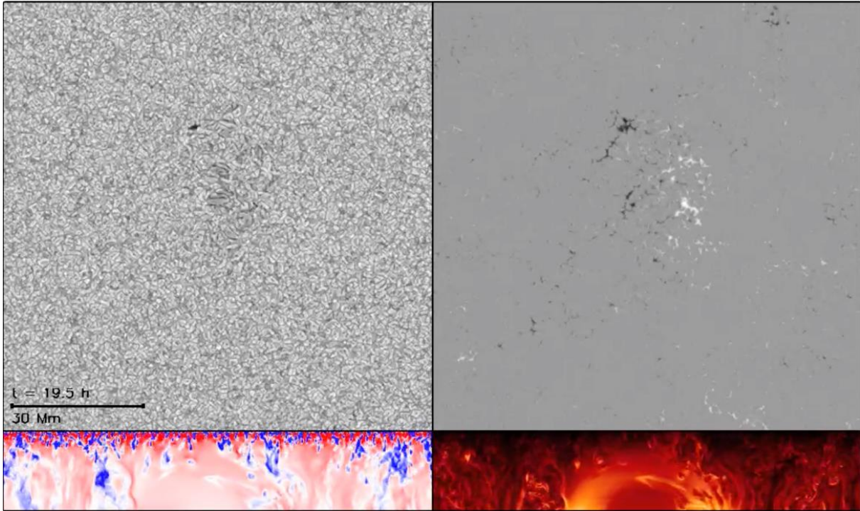
Caption for the movie: The movie shows a simulation of the rise of a magnetic flux concentration through the last 18,000 km below the solar surface. As the flux concentration rises it begins to interact with vigorous subsurface convection. The surface brightness is shown in the top left panel, the vertical magnetic field at the solar surface is shown in the top right panel (black and white shows vertical magnetic fields of opposite polarity). The lower left panel shows the vertical velocity in a vertical plane in the simulation (red for upflows, and blue for downflows), and the lower right panel shows a vertical slice of the magnetic field strength (dark red for strong fields, light yellow for weak fields). Credit: Matthias Rempel @ High Altitude Observatory of the National Center for Atmospheric Research. The National Center for Atmospheric Research is sponsored by the National Science Foundation. Computing time was provided by the NASA High-End Computing (HEC) Program through the NASA Advanced Supercomputing (NAS) Division at Ames Research Center under projects s1325 and s1326.
