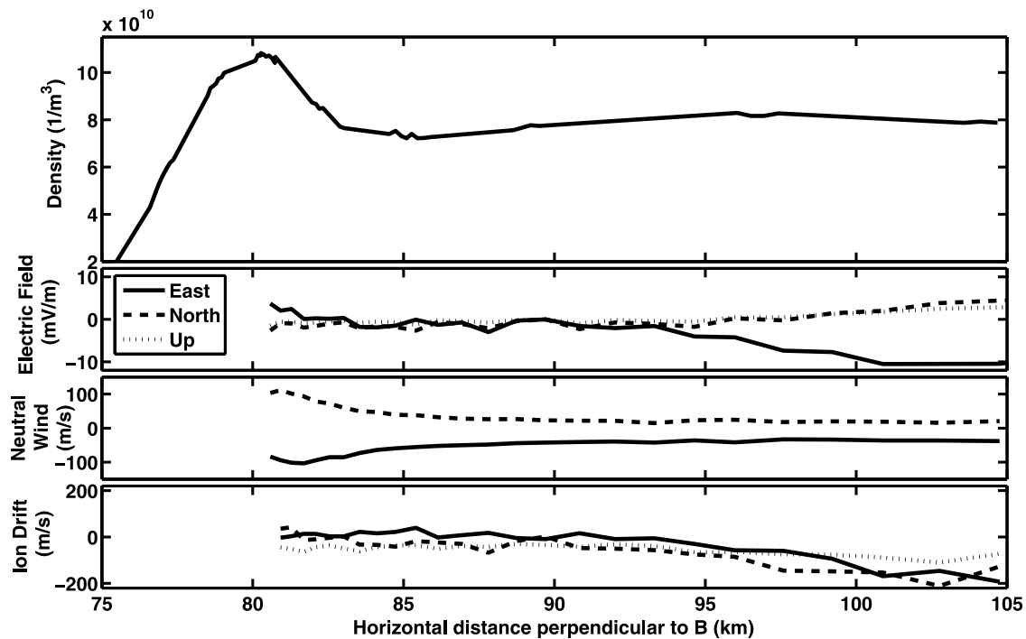
Figure 14. Measured electric field, neutral wind, and plasma density plotted as functions of the distance traveled by the rocket perpendicular to the magnetic field.
