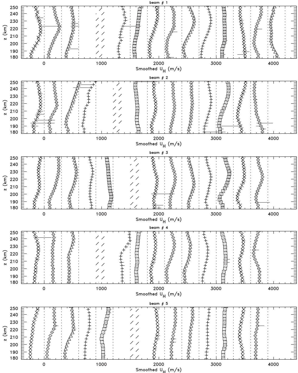
Fig. 13. Extracted background, horizontal, neutral winds, U_H , for beams #1–5, as labeled, smoothed via a nine-point running average to eliminate the small-scale oscillations on vertical scales of 35–40 km. Profiles are offset by 300 m/s. We use the same symbols for the phase lines as in Fig. 8.
