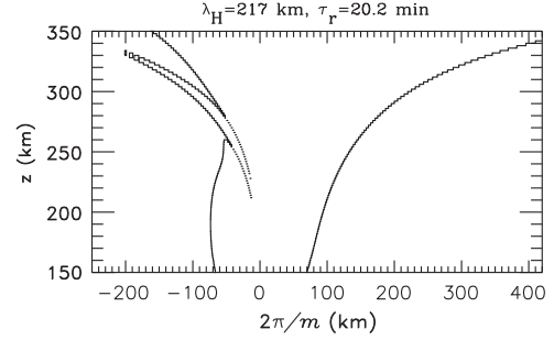
Fig. 1. Solution of the GW dispersion relation, Eq. (1), for a GW with \lambda_H = 217 km and \tau_r = 20.2 min in zero neutral, background winds, U = V = 0 .
