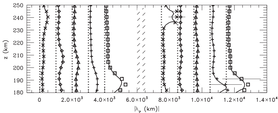
Fig. 17. All 10 |\lambda_z(z)| profiles obtained by ray-tracing GWs #1 and 2 through the extracted winds in Fig. 9a from beam #8 (solid lines). Profiles are offset by 1000 km. As before, GWs #1 and 2 are separated by a hatched region. The dot lines show \lambda_z = 0 for each constant phase line. We use the same symbols for the phase lines as in Fig. 8.
