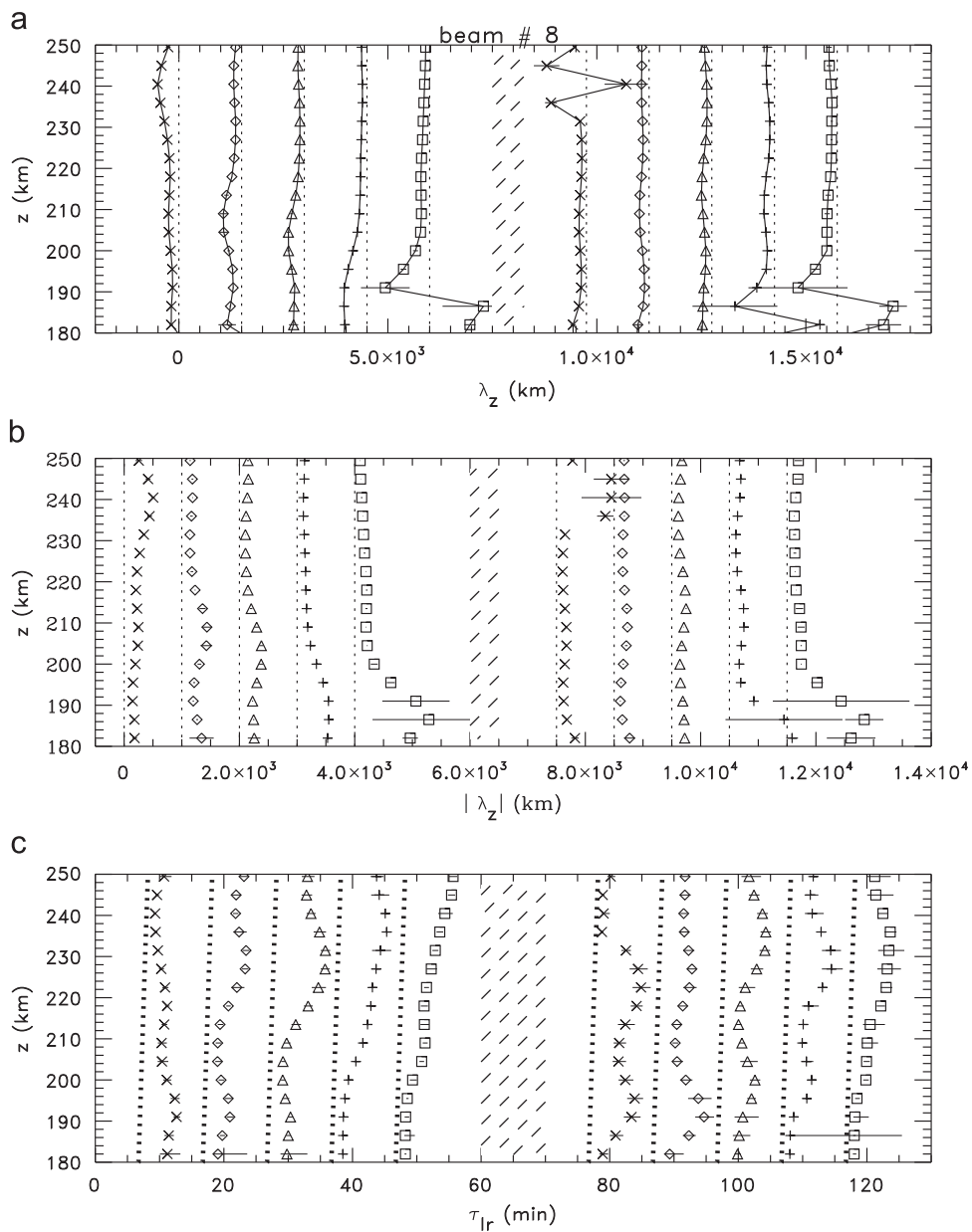
Fig. 8. (a) Values of \lambda_z(z) computed from Eq. (29) using the solid lines in Fig. 7 for both GWs in beam #8. The \lambda_z(z) profiles are offset by 1500 km. The results along the first, second, third, fourth and fifth constant wave phase lines are shown as \times 's, diamonds, triangles, +s, and squares, respectively. The following five phase lines repeat these symbols. The dot lines show \lambda_z = 0 for each constant phase line. The hatched regions with dashed lines separate GWs #1 and 2. (b) Same as in (a), but showing |\lambda_z(z)| instead. The profiles are offset by 1000 km. (c) Computed values of the intrinsic period via solving Eq. (1) iteratively. Profiles are offset by 10 min, and use the same symbols as in (a). The buoyancy period, 2\pi/N , is shown as dotted lines.
