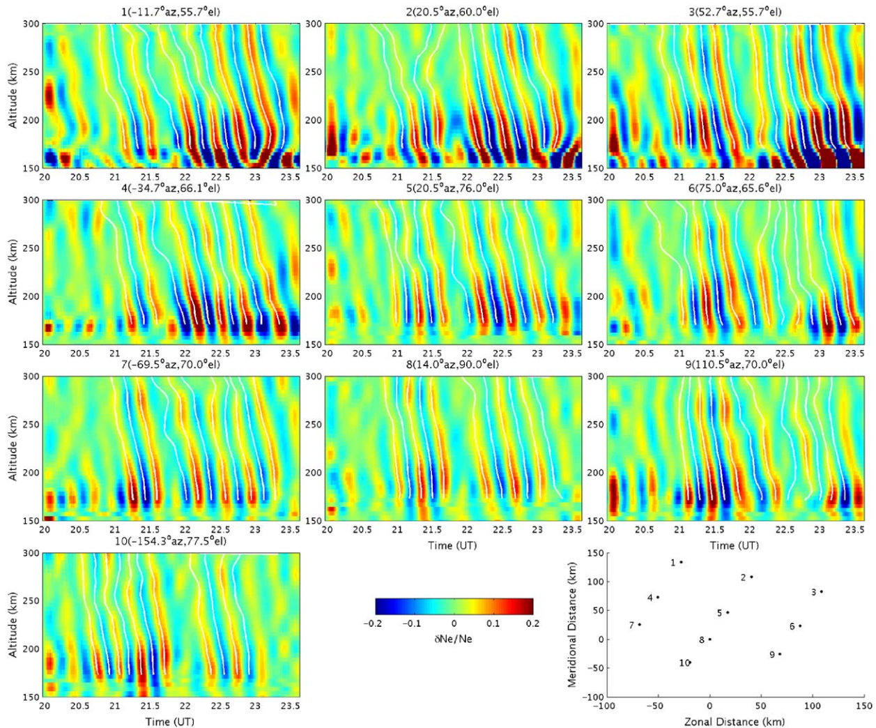
Fig. 2. Electron density fractional perturbations for all 10 beams as a function of time and altitude on 13 December 2006. The lower right panel shows beam positions at an altitude of \sim 200 km.
