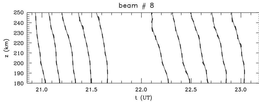
Fig. 7. Times where the GW phases are maximum as a function of altitude for beam #8 (dash lines). Three-point running average of the same times (solid lines).
