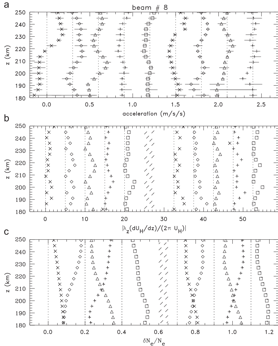
Fig. 11. (a) Neutral, background wind accelerations, \Delta U_H/\Delta t , using the data in Figs. 7 and 9a. The acceleration profiles between the first and second (1–2), second and third (2–3), etc., wave phases are shown as \times 's, diamonds, triangles, + 's, squares, \times 's, diamonds, triangles, and + 's, respectively. Profiles are offsetted by 0.3 m/s 2 . (b) |\lambda_z/(2\pi U_H)(dU_H/dz)| . Profiles are offsetted by 5 . (c) \delta N_e/N_e for GWs #1 and 2 along the constant wave phase lines. Odd-numbered profiles are offsetted by 0.2 . The symbols in (b) and (c) are the same as in Fig. 8.
